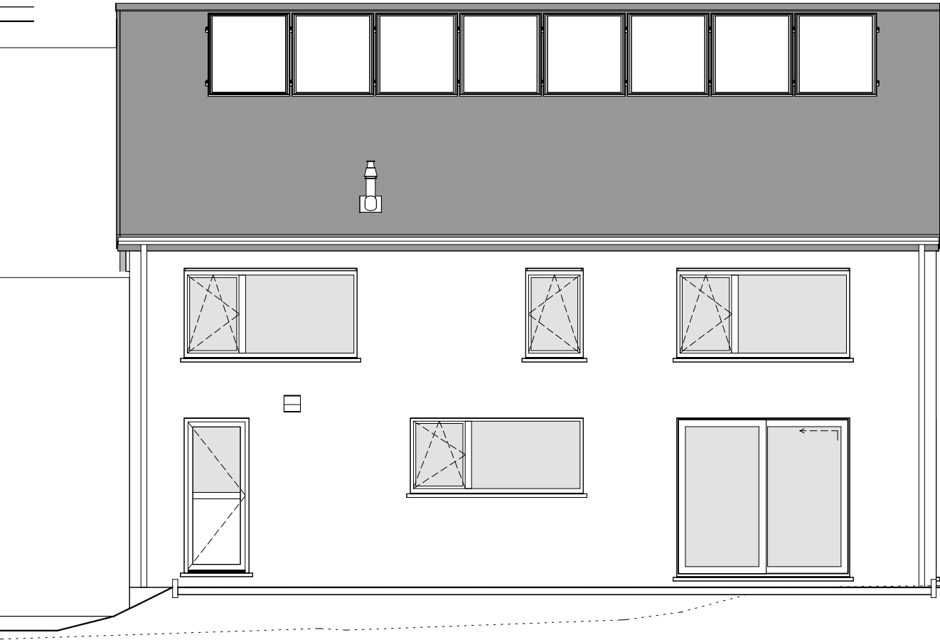
FACADE ARRIERE
