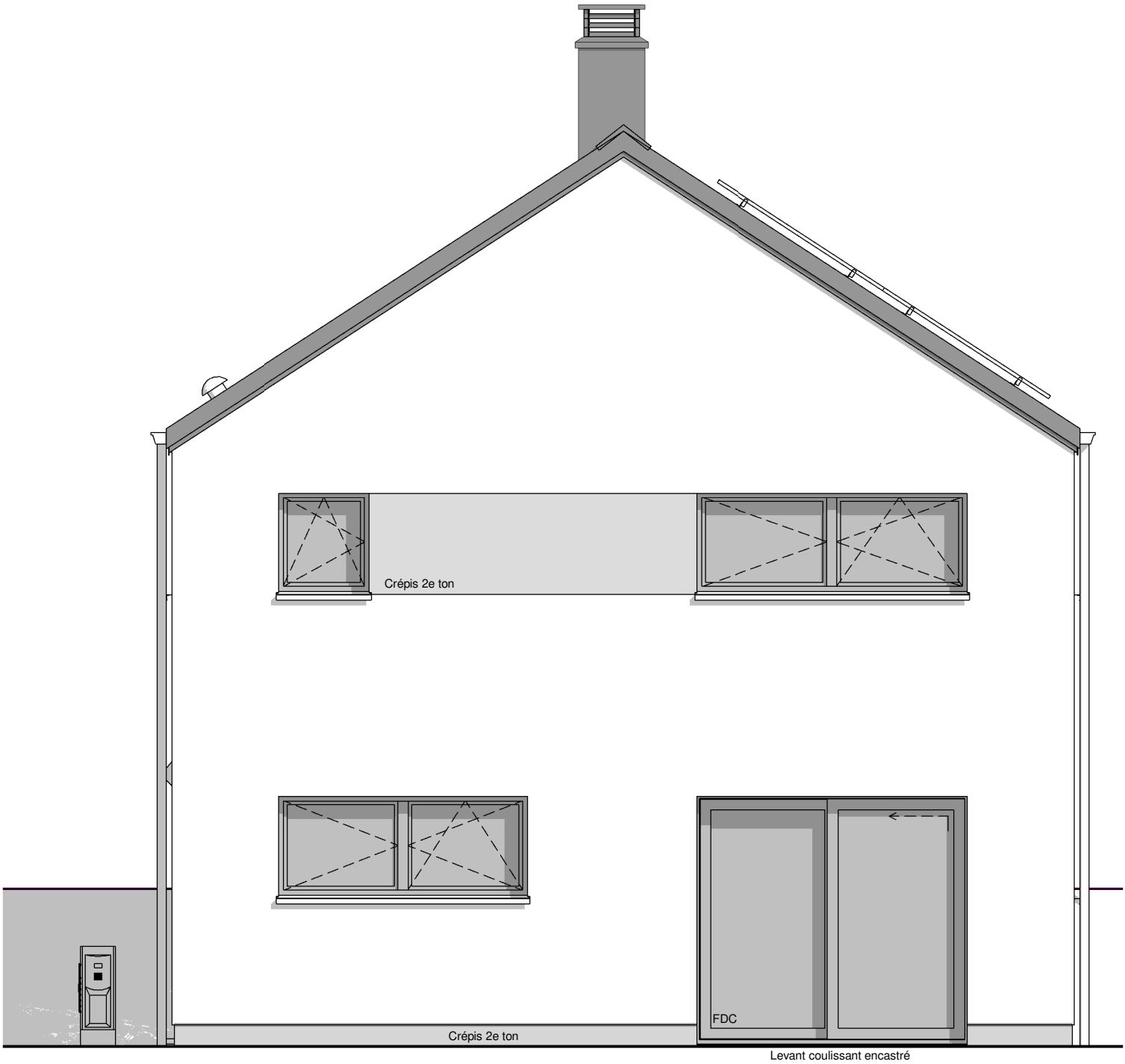
PIGNON ARRIERE
