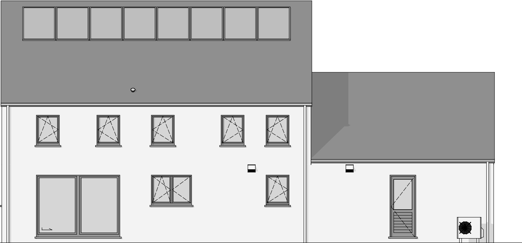
FACADE ARRIERE
