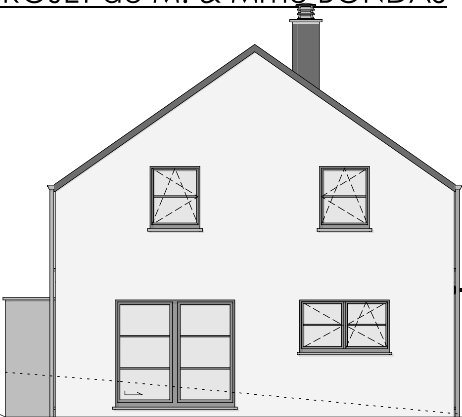
PIGNON ARRIERE
