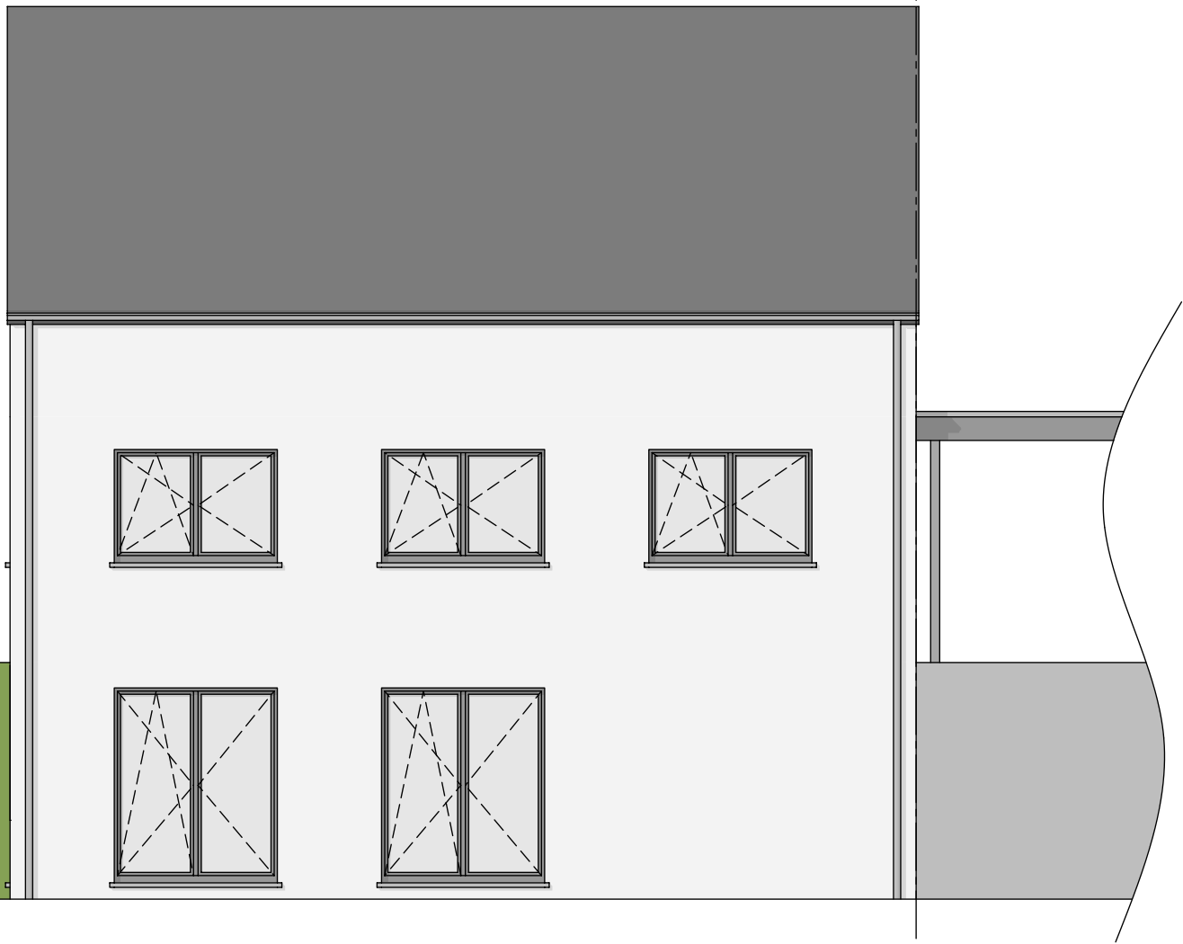
FACADE ARRIERE
