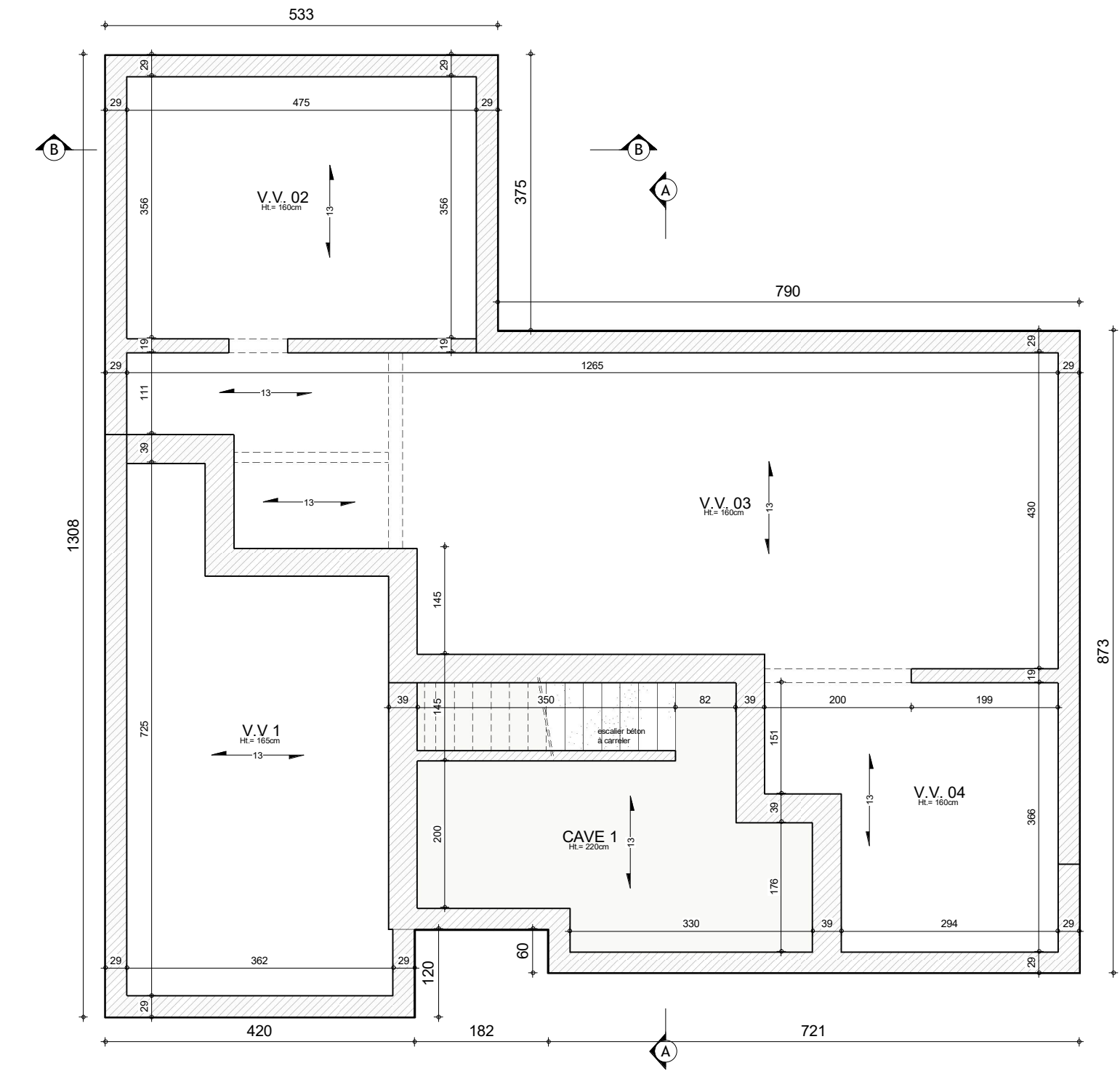
CAVES
