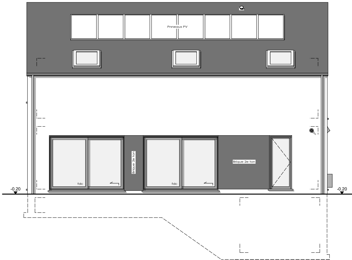
FACADE ARRIERE
