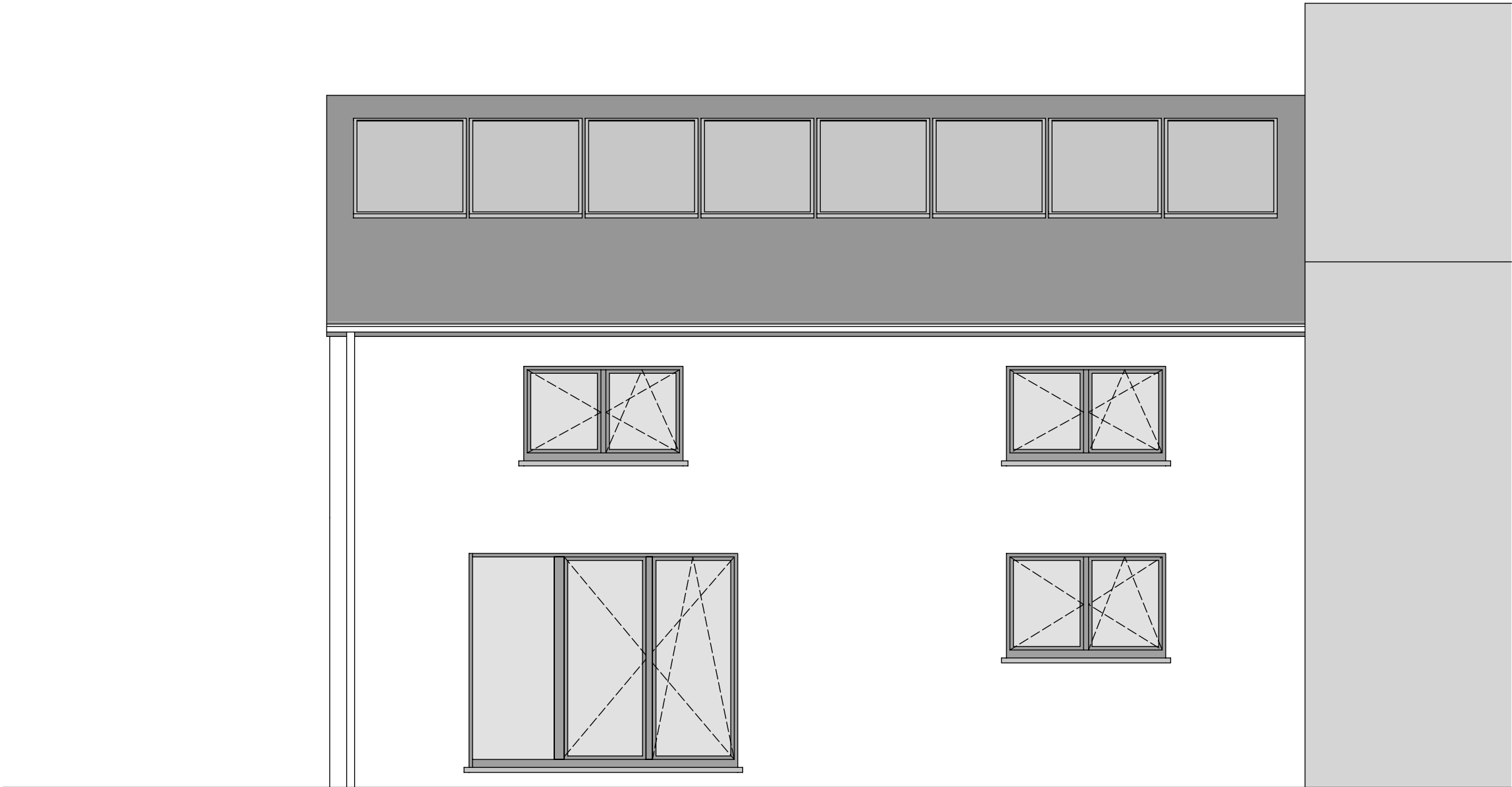
FACADE ARRIERE
