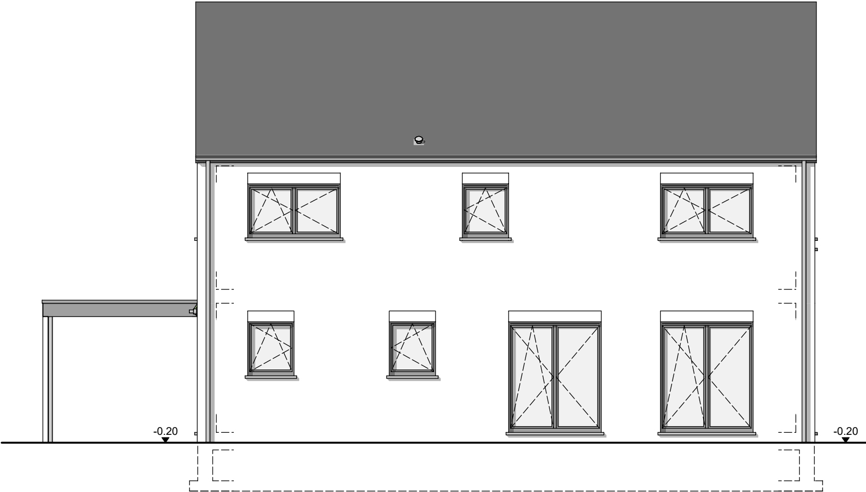
FACADE ARRIERE
