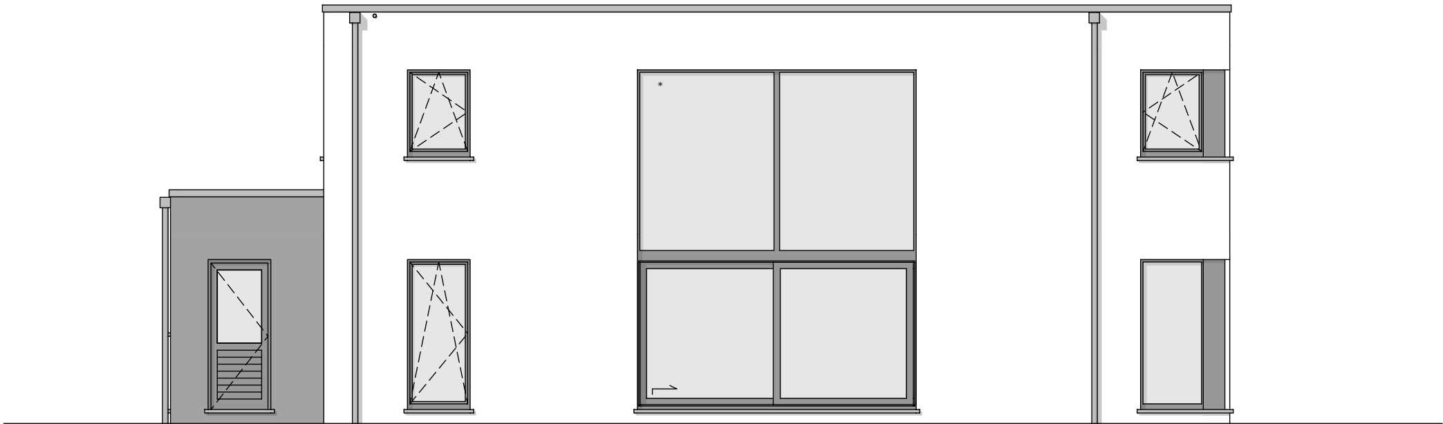
FACADE ARRIERE
