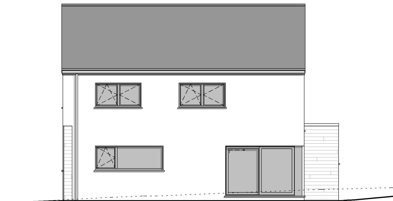
FACADE ARRIERE
