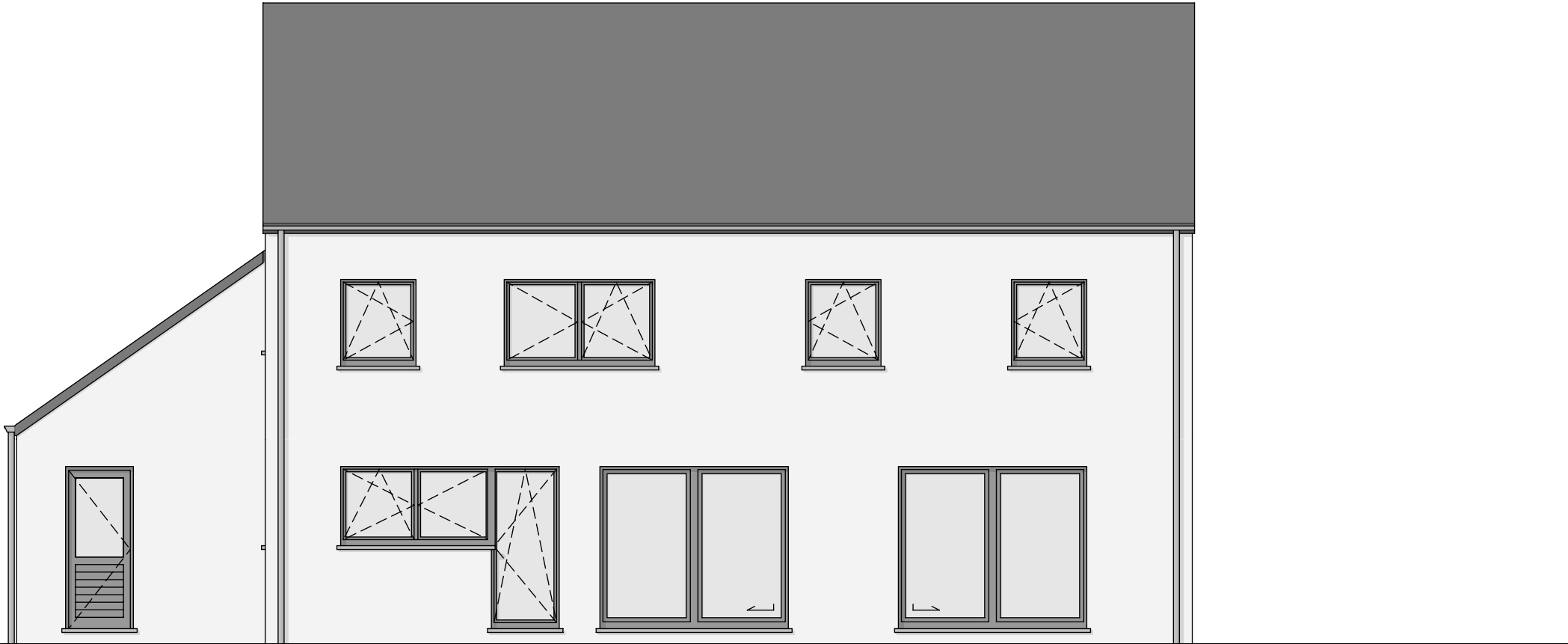
FACADE ARRIERE
