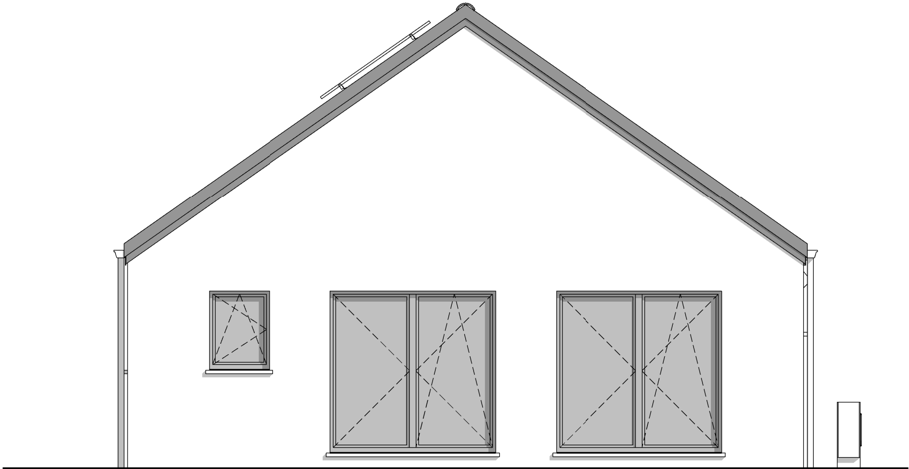
FACADE ARRIERE
