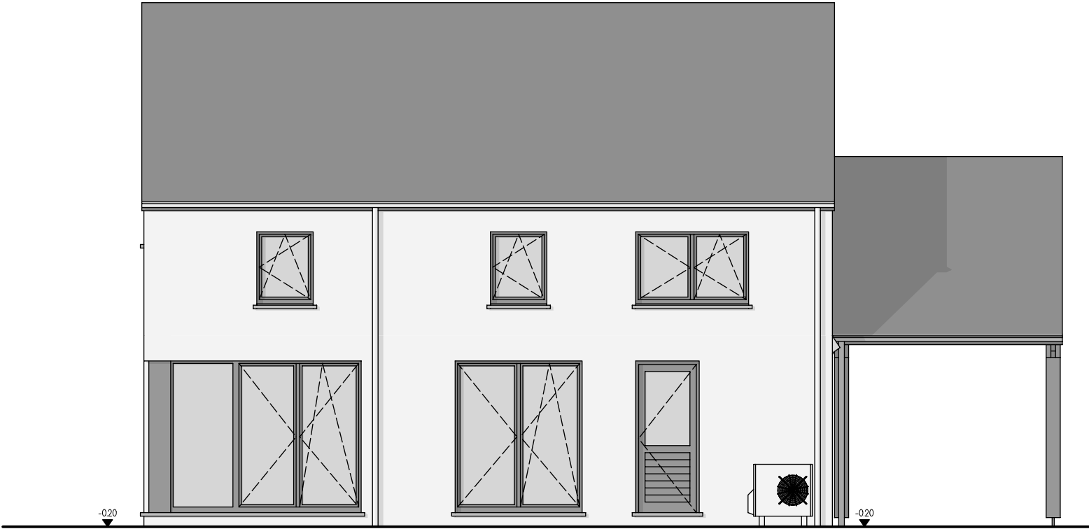
FACADE ARRIERE
