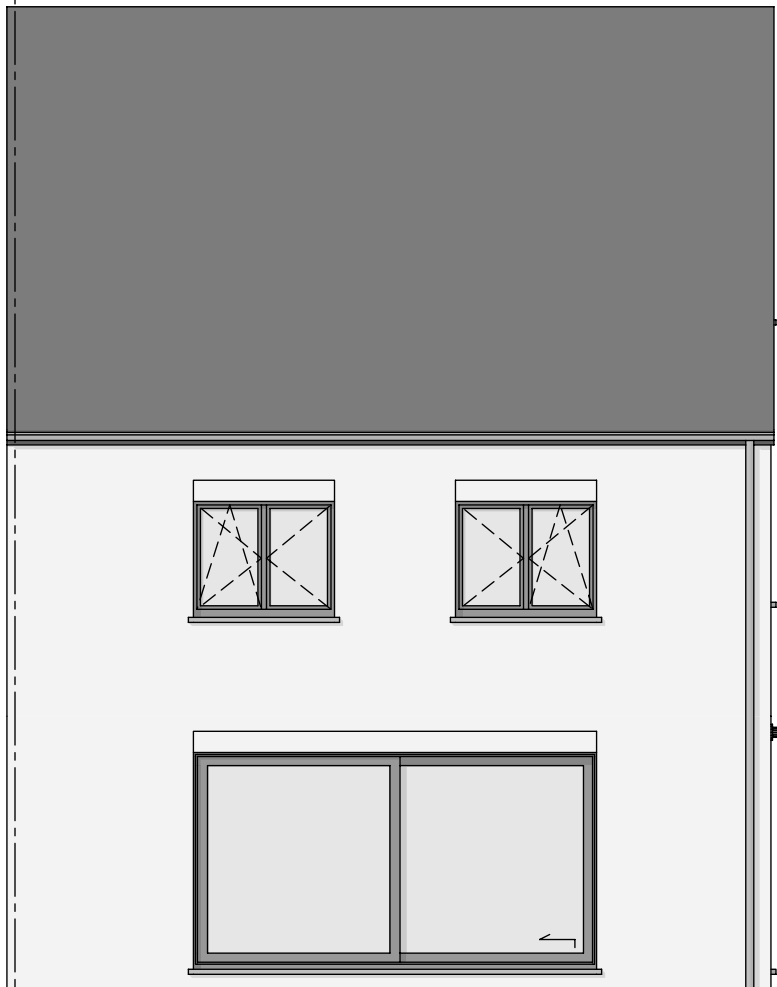
FACADE ARRIERE
