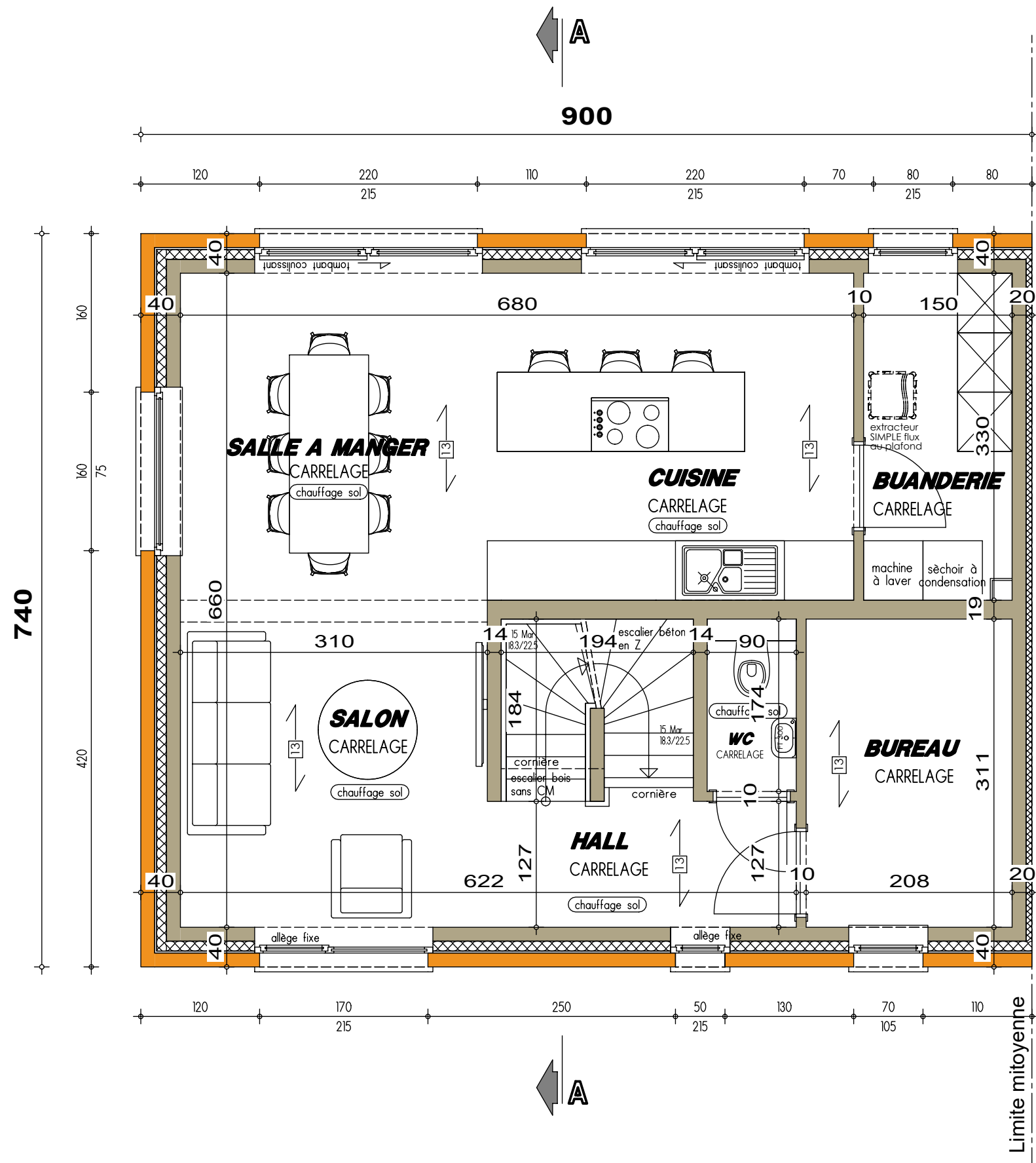
PLAN REZ-DE-JARDIN
