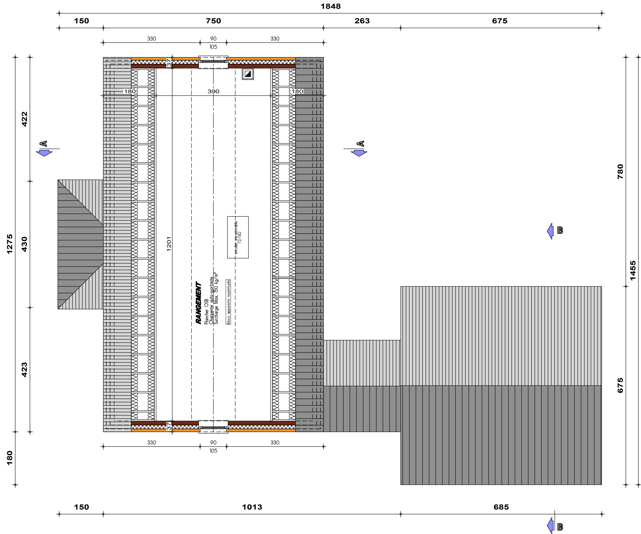
PLAN COMBLES
