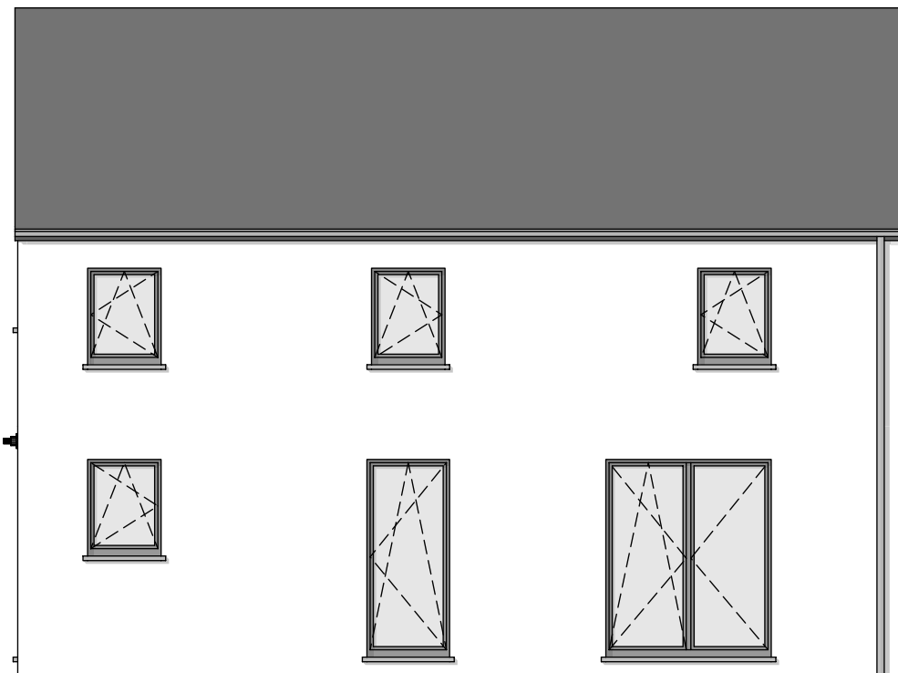
FACADE ARRIERE
