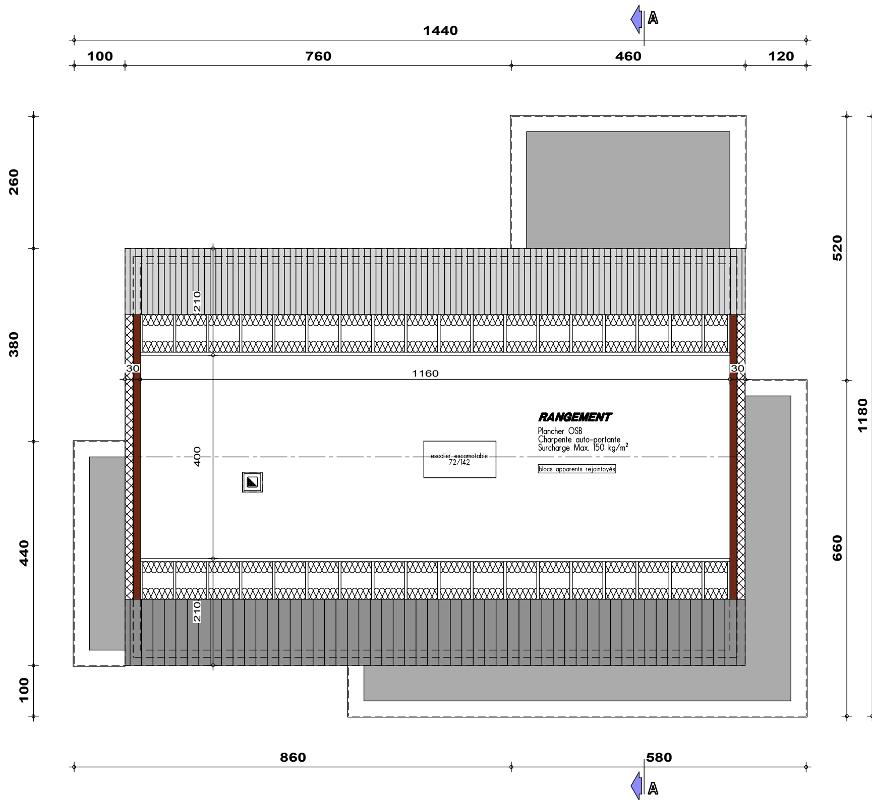
PLAN COMBLES
