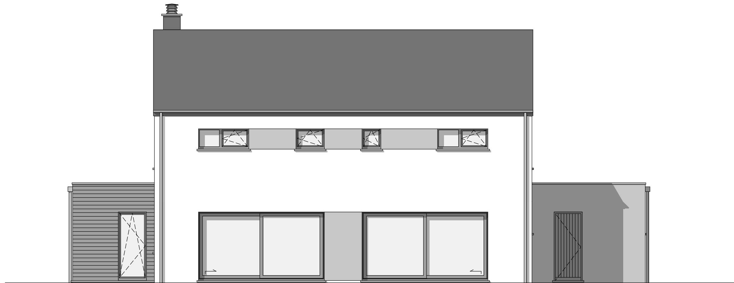
FACADE ARRIERE
