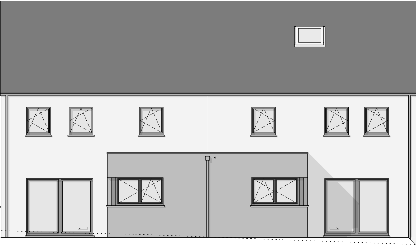
FACADE ARRIERE
