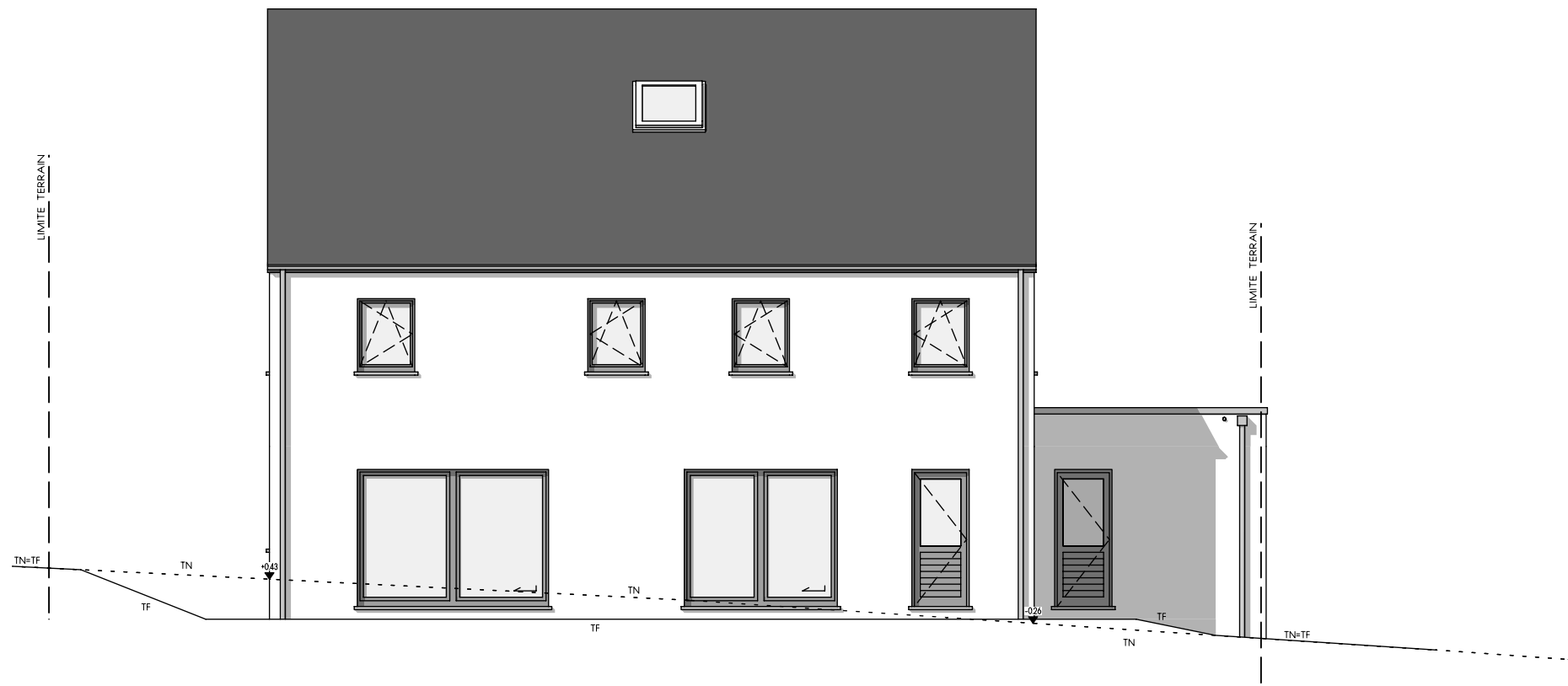
FACADE ARRIERE
