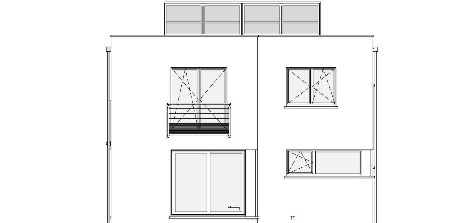
FACADE ARRIERE
