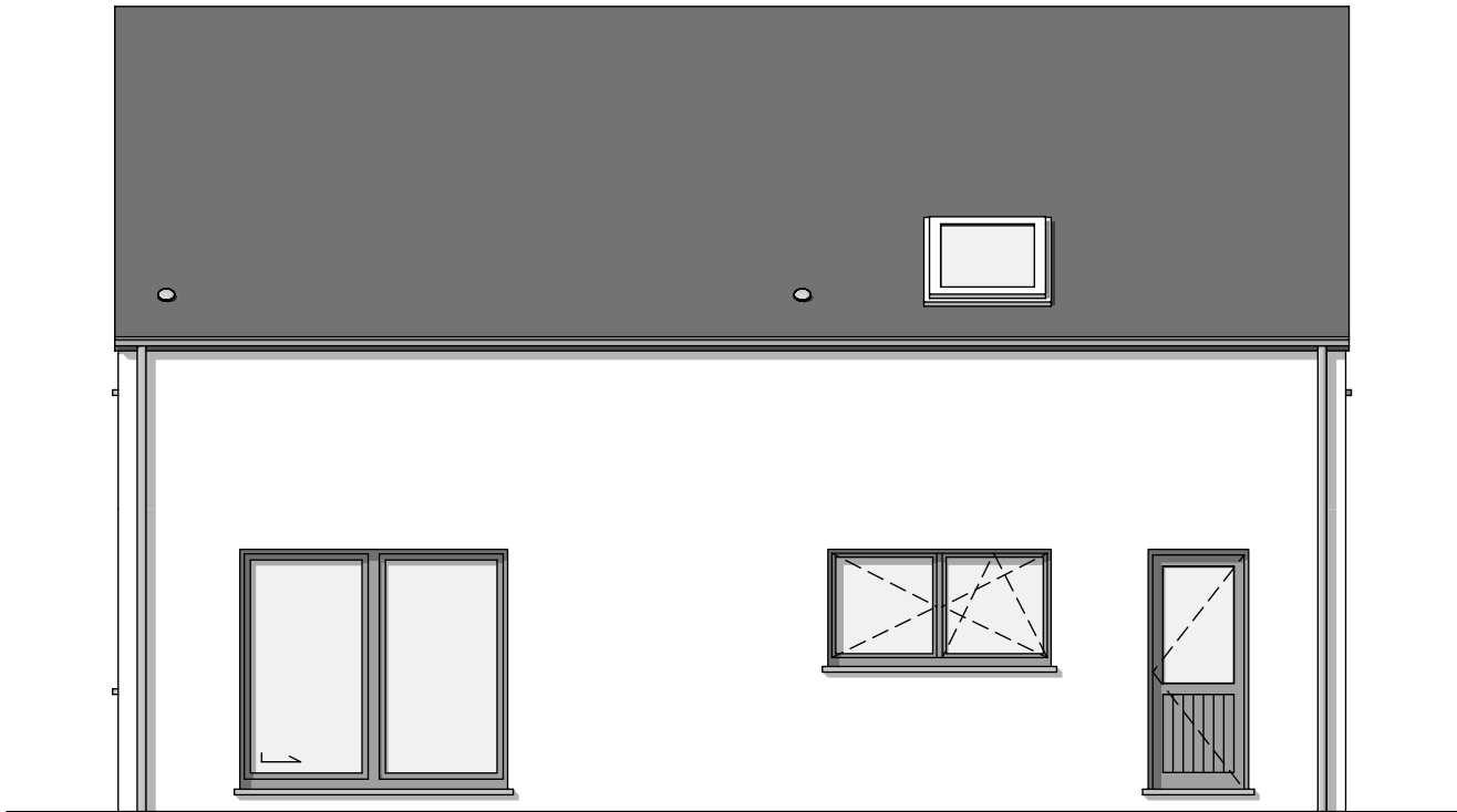
FACADE ARRIERE
