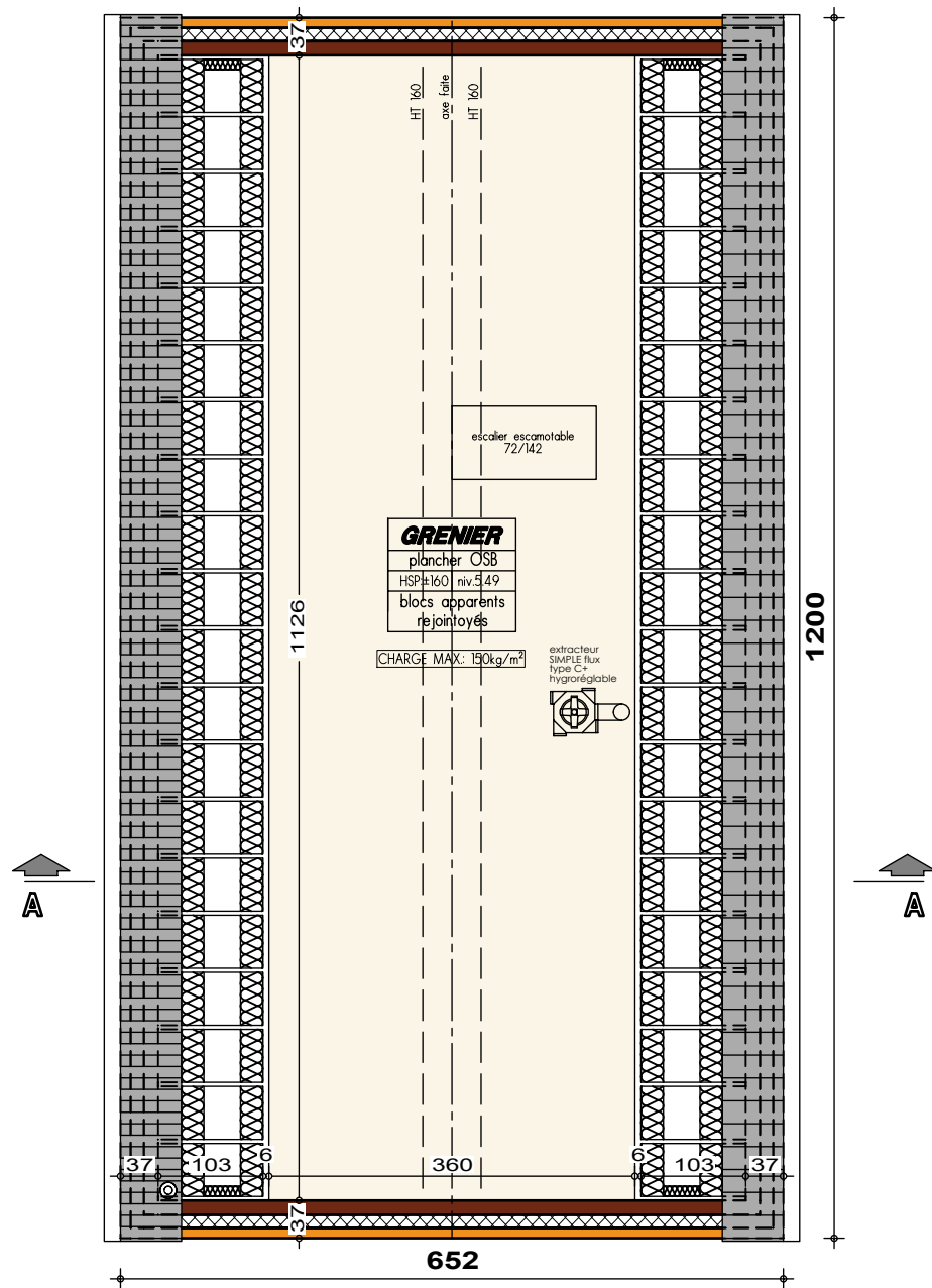
PLAN COMBLES
