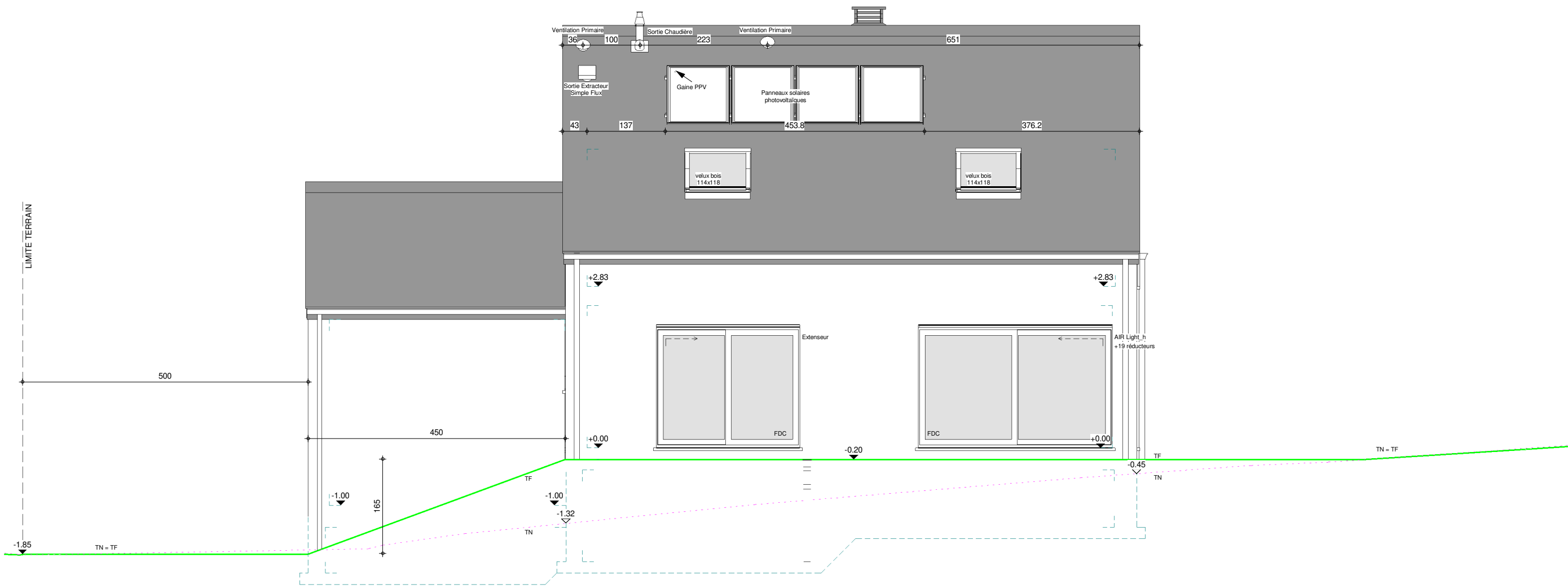
FACADE ARRIERE
