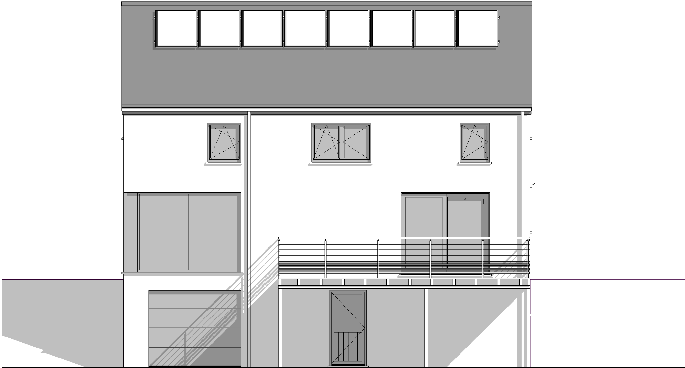
FACADE ARRIERE
