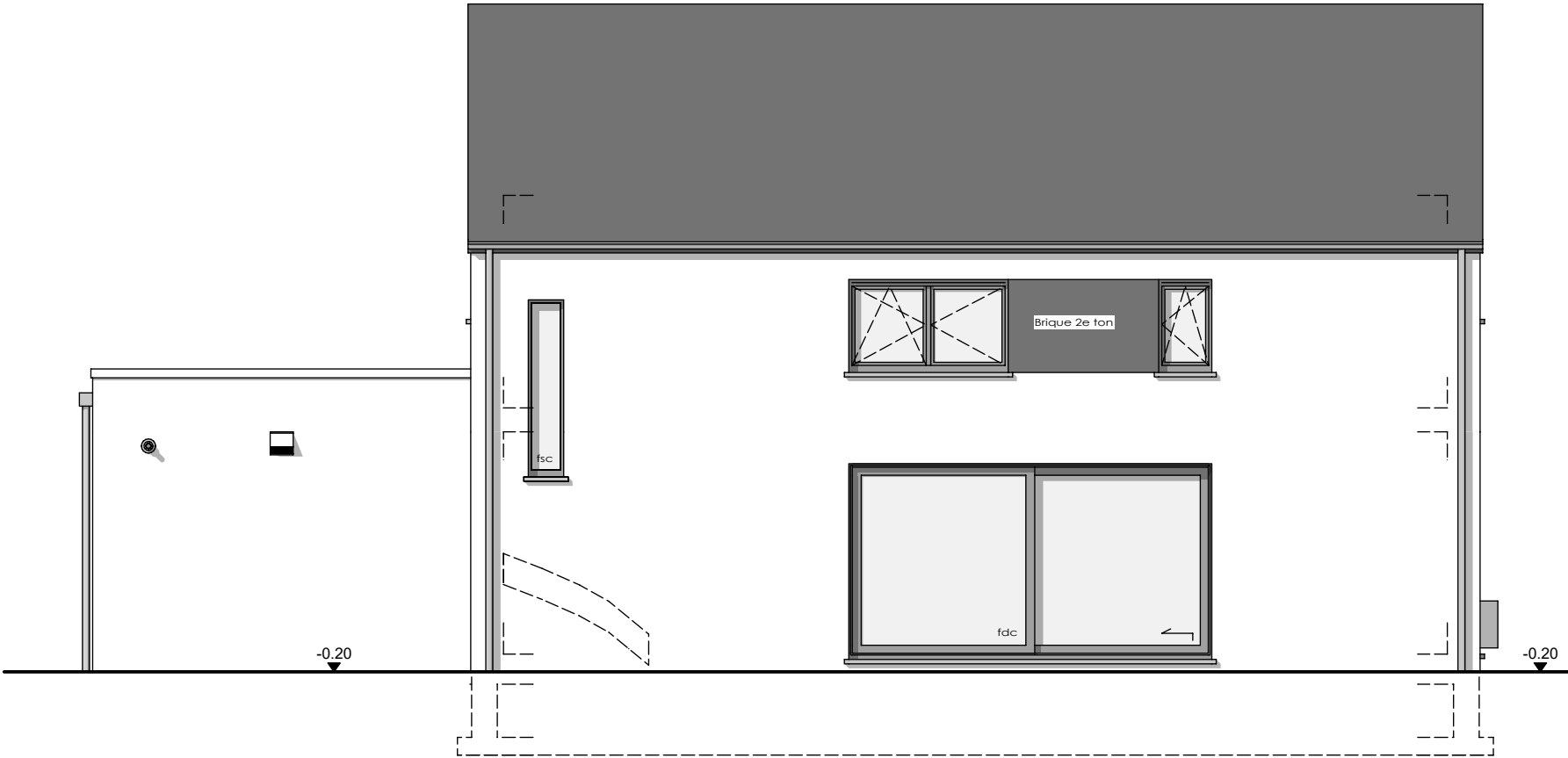
FACADE ARRIERE
