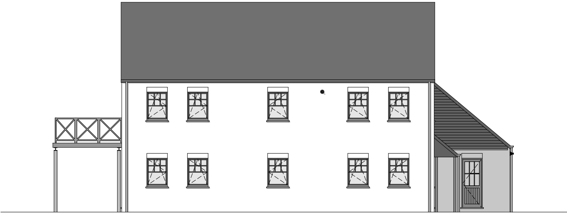
FACADE ARRIERE
